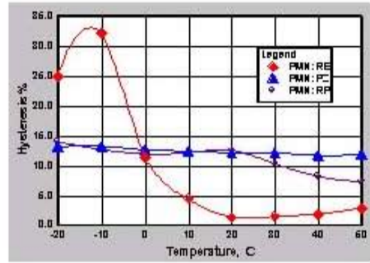
PMN Family Hysteresis Response
