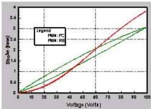
PMN Family Gain Response
