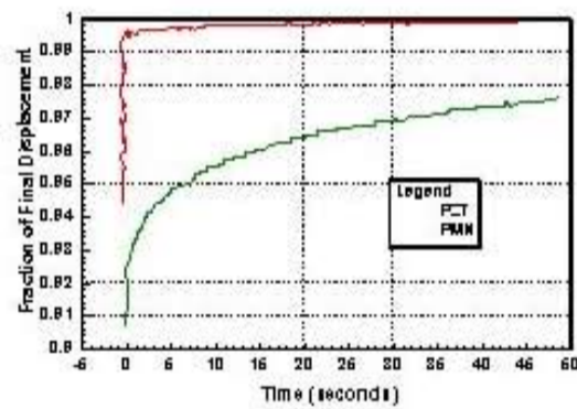
Creep Comparison: PMN versus PZT
