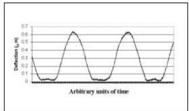
XiCRI Electrostrictive Response at 65 K
