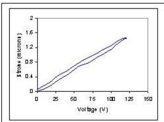
XiCRI Electrical Hysteresis at 65 K
