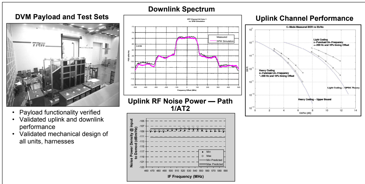
Figure 5. DVM Payload Integration Complete
