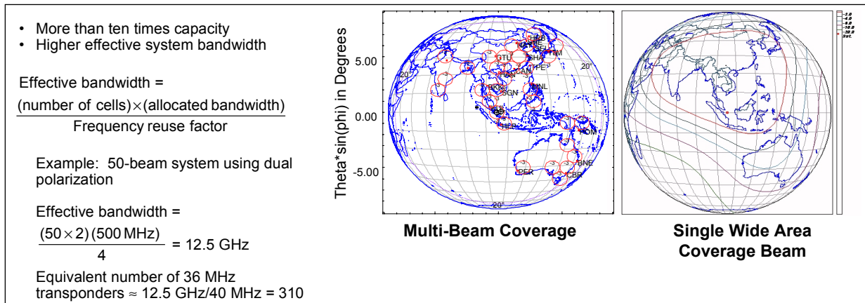
Figure 7. Higher Capacity Through Frequency Reuse 01S02418-K-040-R2-154
