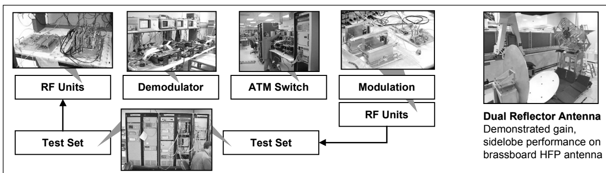
Figure 4. End-to-End Hardware Functional Prototype Testbed Demonstrated Payload/System
