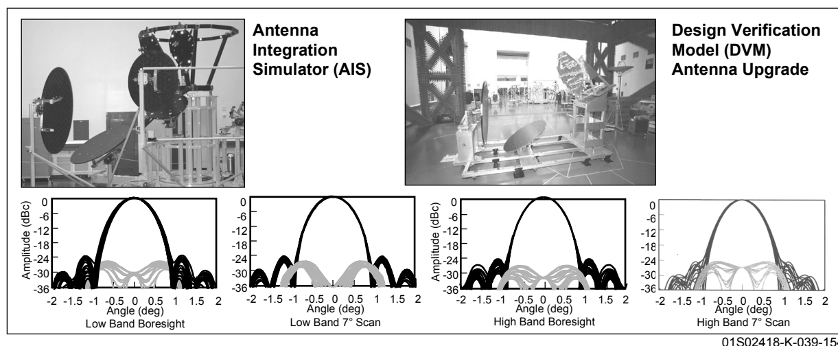
Figure 6. Antenna Integration Simulator and Design Verification Model
