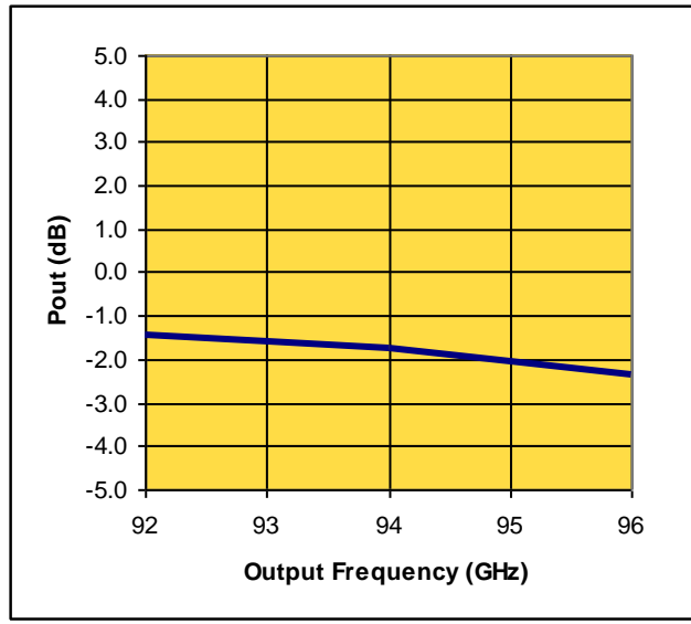
Output Power
