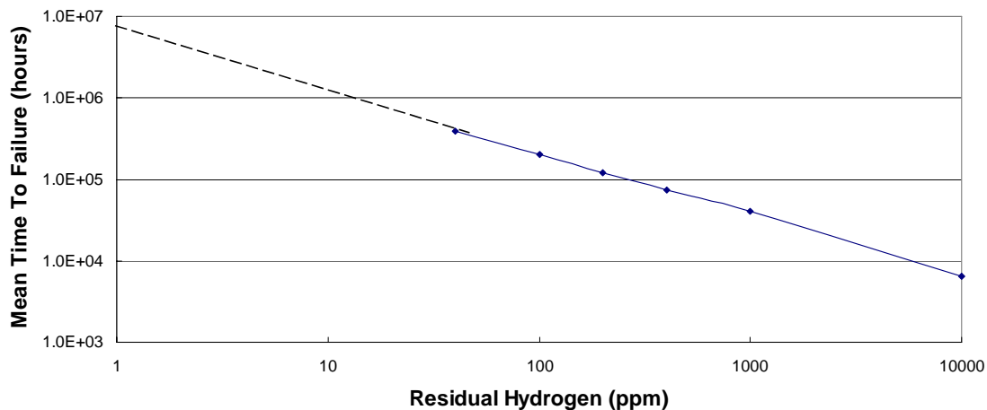
Figure 2. GaAs HEMT Reliability vs. Residual Hydrogen at 60C baseplate temperature. Note that baseplate temperature is used instead of junction temperature for reliability model of H2 effect
