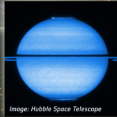
Image: Hubble Space Telescope
