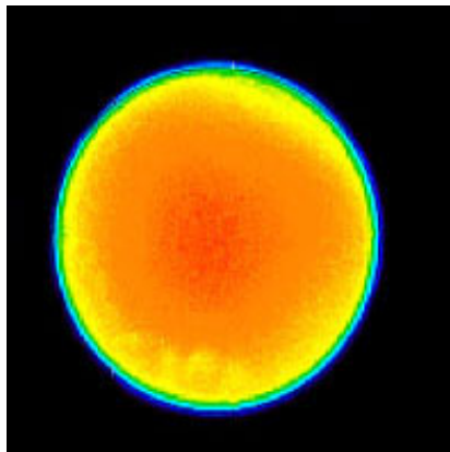
4mm, 0.6% Dopant Nd:YAG Rod
